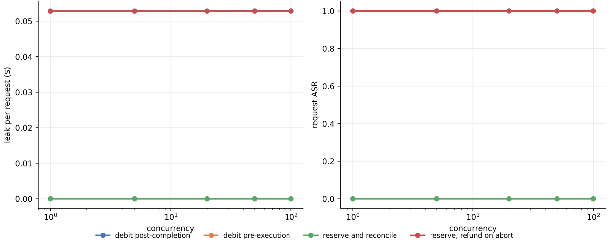
Figure 4: M1 negative result. Request volume is held constant at 20 requests per cell while concurrency varies from 1 to 100 ( x -axis, log scale); the y -axis is mean leakage per request and request-level attack success. Both are invariant across the range, which is the empirical basis for treating commitment timing as a per-request rather than a contention-driven defect. Holding volume constant is what prevents traffic level from masquerading as vulnerability.
