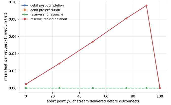
Figure 3: M1 leakage against abort position, deterministic generator, concurrency 1, medium price tier, 20 requests per cell. The x-axis is the fraction of the response streamed before the client disconnects; the y-axis is mean leakage per request in scenario dollars, i.e., delivered value minus net committed debit. Vulnerable architectures peak just before the commit would have fired and collapse to $0 at completion, when it does fire; safe architectures stay at $0 throughout. All values are empirical. Error bars are within-cell standard deviations and are zero at this concurrency.
