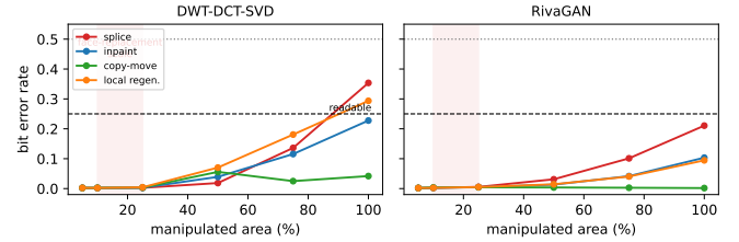
Fig. 4. Mean BER against manipulated area for four manipulation families. The shaded band is realistic face-replacement coverage; the dashed line is the readability threshold.
