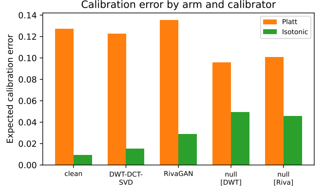
Fig. 5. ECE by arm under each calibrator. Isotonic shows attenuation degrading calibration; Platt shows the opposite, resolved by its badly misspecified clean-arm baseline (0.1273, 13 \times isotonic’s).
