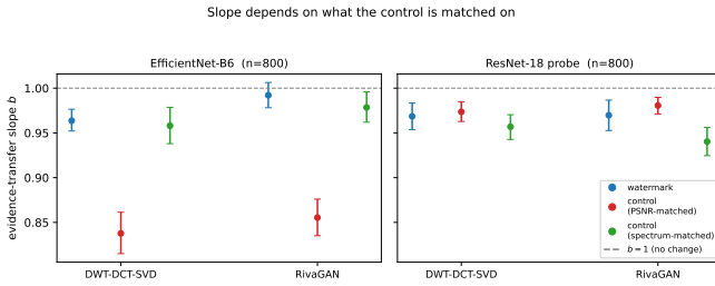
Fig. 3. Slope of each arm with bootstrap intervals. On EfficientNet-B6 the PSNR-matched control sits far below b = 1 while the watermark and the spectrum-matched control sit together near it.
