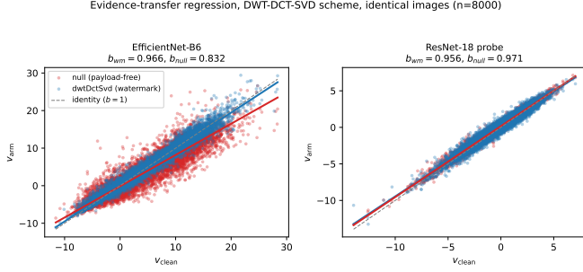
Fig. 1. Evidence-transfer regression on the same 8,000 images, DWT-DCT-SVD scheme. EfficientNet-B6 (left) shows the null arm (red) pulled below identity while the watermark (blue) tracks it; the ResNet-18 probe (right) shows the opposite ordering.
