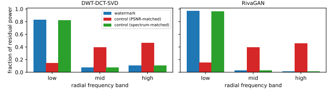
Fig. 2. The PSNR-matched control is spectrally inverted relative to the watermark it stands in for; the spectrum-matched control is not.
