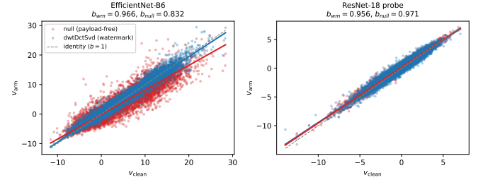
Fig. 1. Evidence-transfer regression on the same 8,000 images, DWT-DCT-SVD scheme. EfficientNet-B6 (left) shows the null arm (red) pulled below identity while the watermark (blue) tracks it; the ResNet-18 probe (right) shows the opposite ordering.
