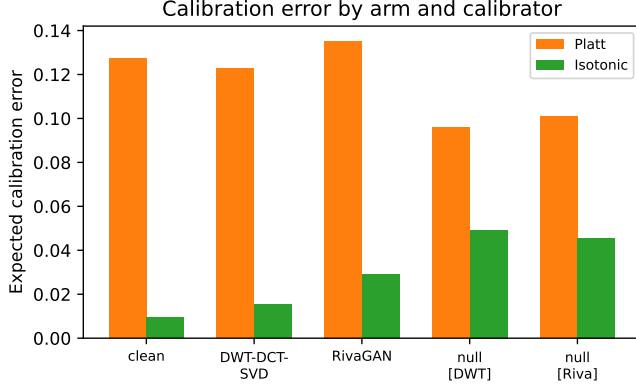
Fig. 5. ECE by arm under each calibrator. Isotonic shows attenuation degrading calibration; Platt shows the opposite, resolved by its badly misspecified clean-arm baseline (0.1273, 13 \times isotonic’s).
