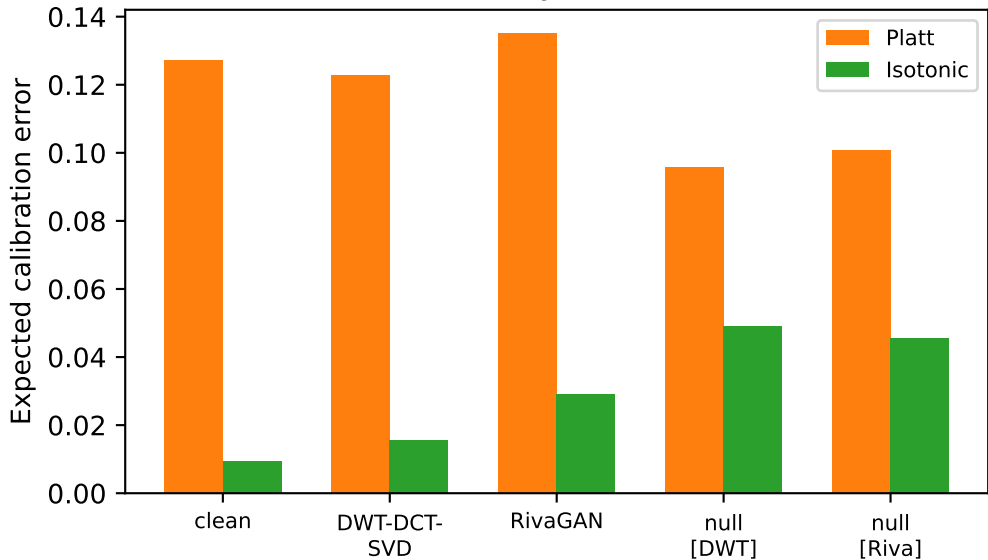
Calibration error by arm and calibrator
