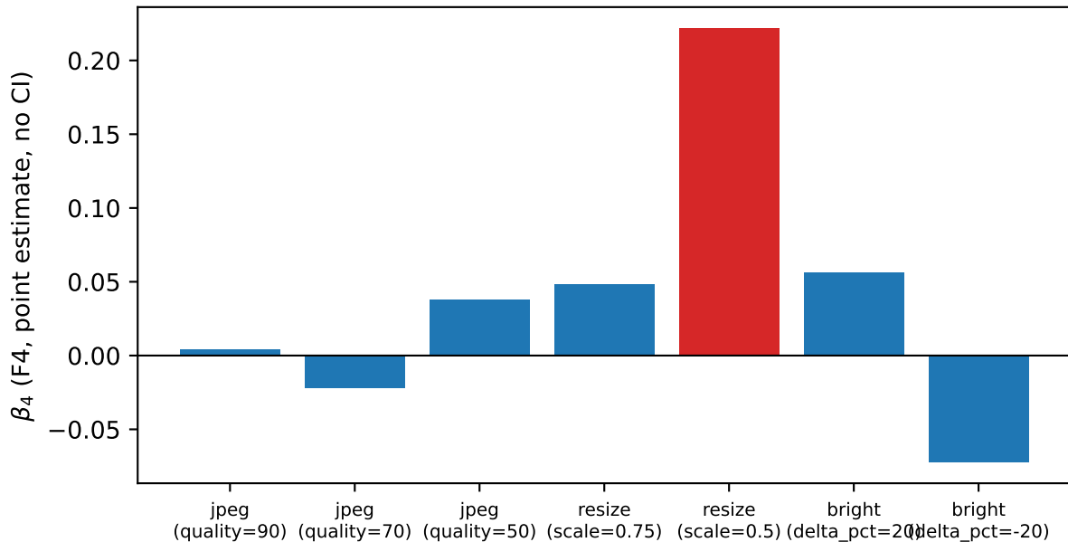
Interference coefficient by transform, n=400 (first look)
