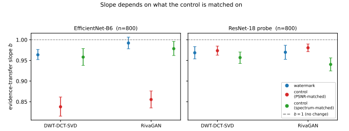
Fig. 3. Slope of each arm with bootstrap intervals. On EfficientNet-B6 the PSNR-matched control sits far below b = 1 while the watermark and the spectrum-matched control sit together near it.
