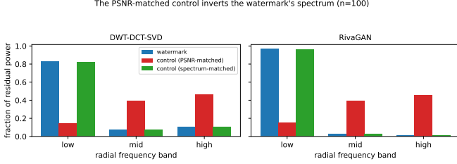
Fig. 2. The PSNR-matched control is spectrally inverted relative to the watermark it stands in for; the spectrum-matched control is not.
