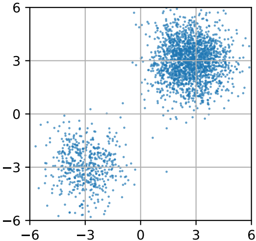
Data distribution
