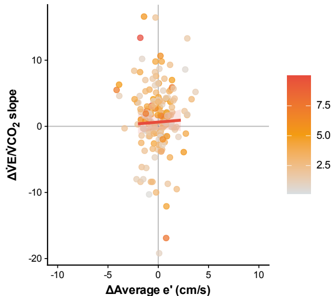
Figure S4. Exploratory within-patient longitudinal coupling between change in average mitral annular e' and change in cardiopulmonary performance. Points represent follow-up studies relative to the first paired observation with both e' and the given outcome available. Point color encodes years since the paired baseline; solid lines and shaded bands show the adjusted mixed-model association.
