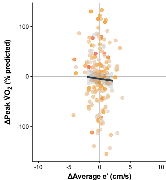
Figure S4. Exploratory within-patient longitudinal coupling between change in average mitral annular e' and change in cardiopulmonary performance. Points represent follow-up studies relative to the first paired observation with both e' and the given outcome available. Point color encodes years since the paired baseline; solid lines and shaded bands show the adjusted mixed-model association.
