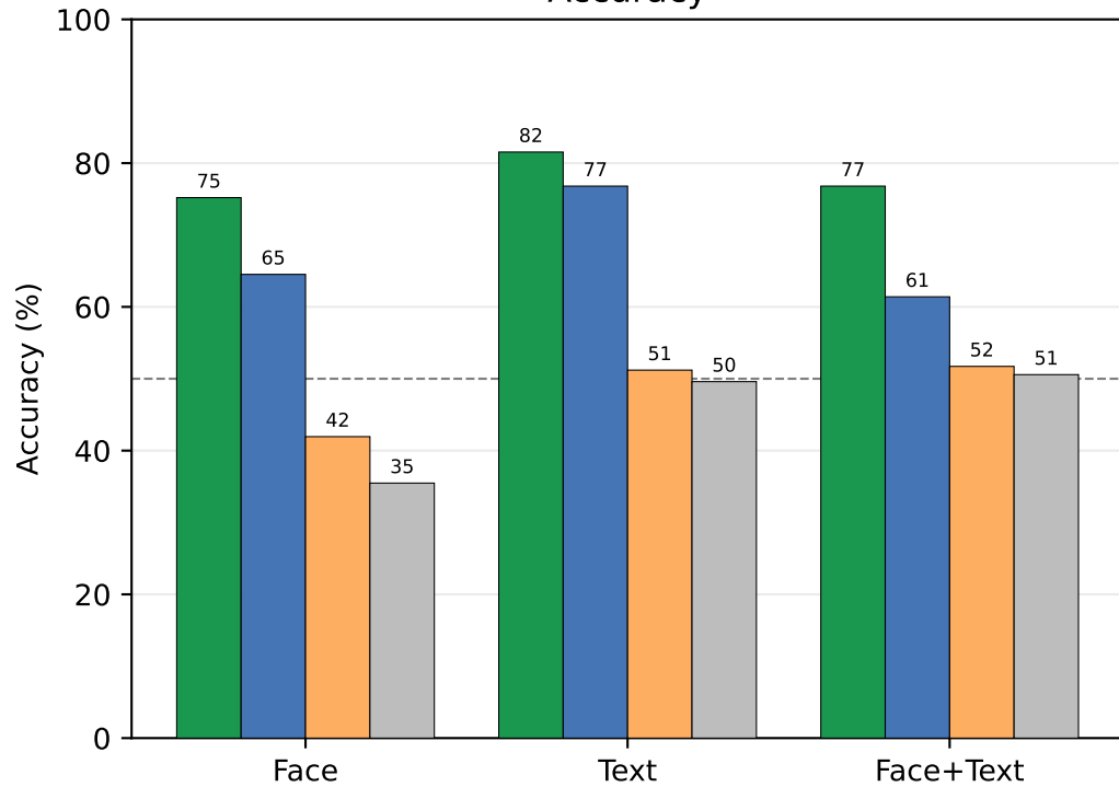
Accuracy
