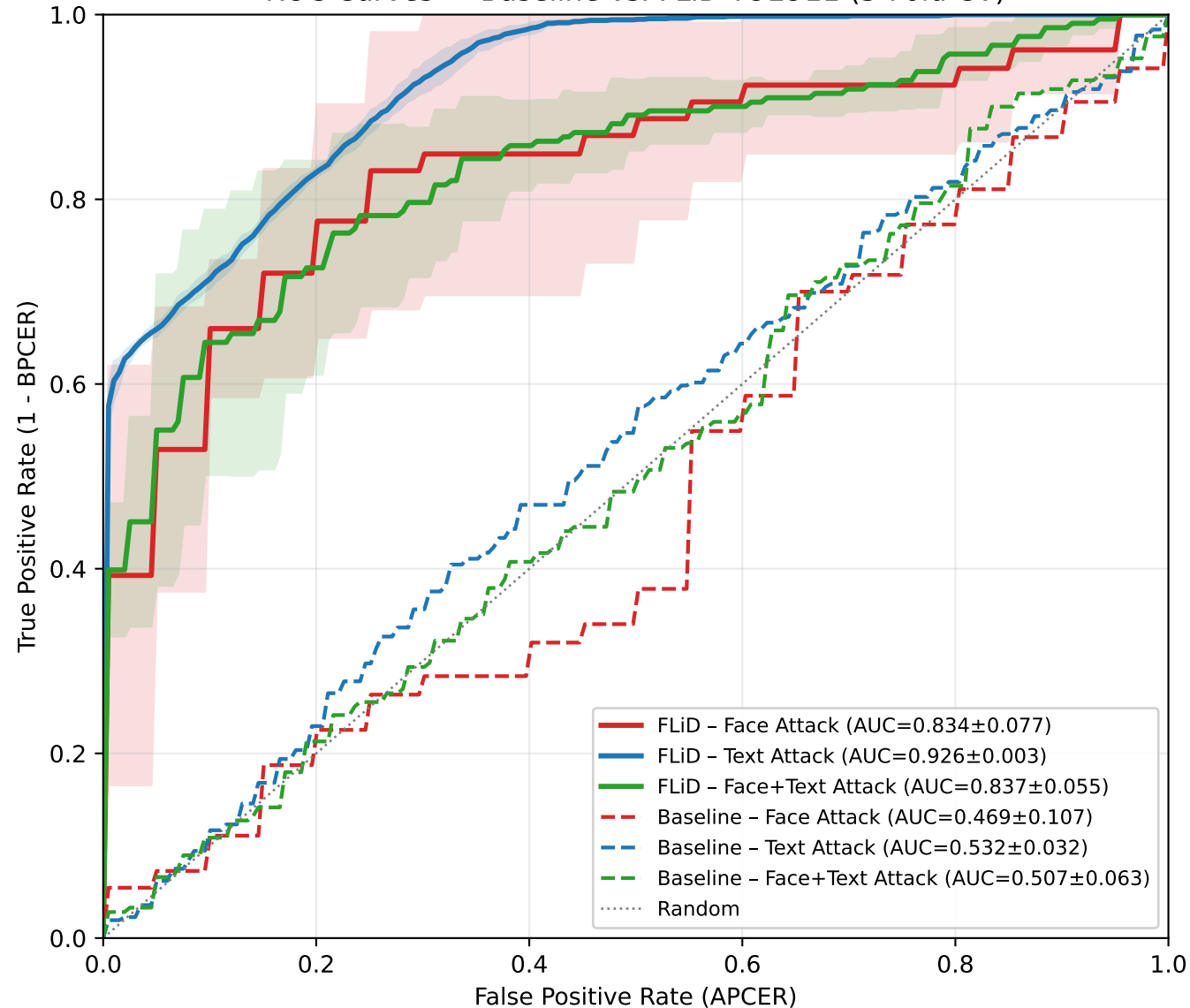
ROC Curves — Baseline vs. FLiD YOLO11 (5-Fold CV)
