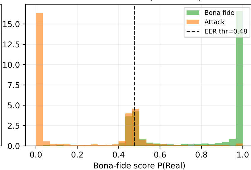
Baseline - Text Attack (AUC=0.532)
