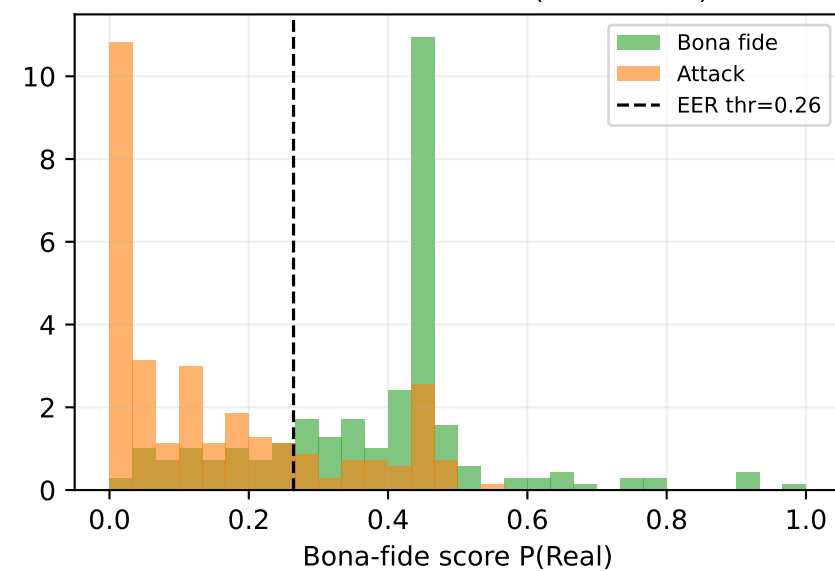
Baseline - Face+Text Attack (AUC=0.507)
