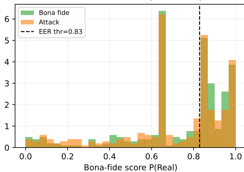
Baseline - Text Attack (AUC=0.532)
