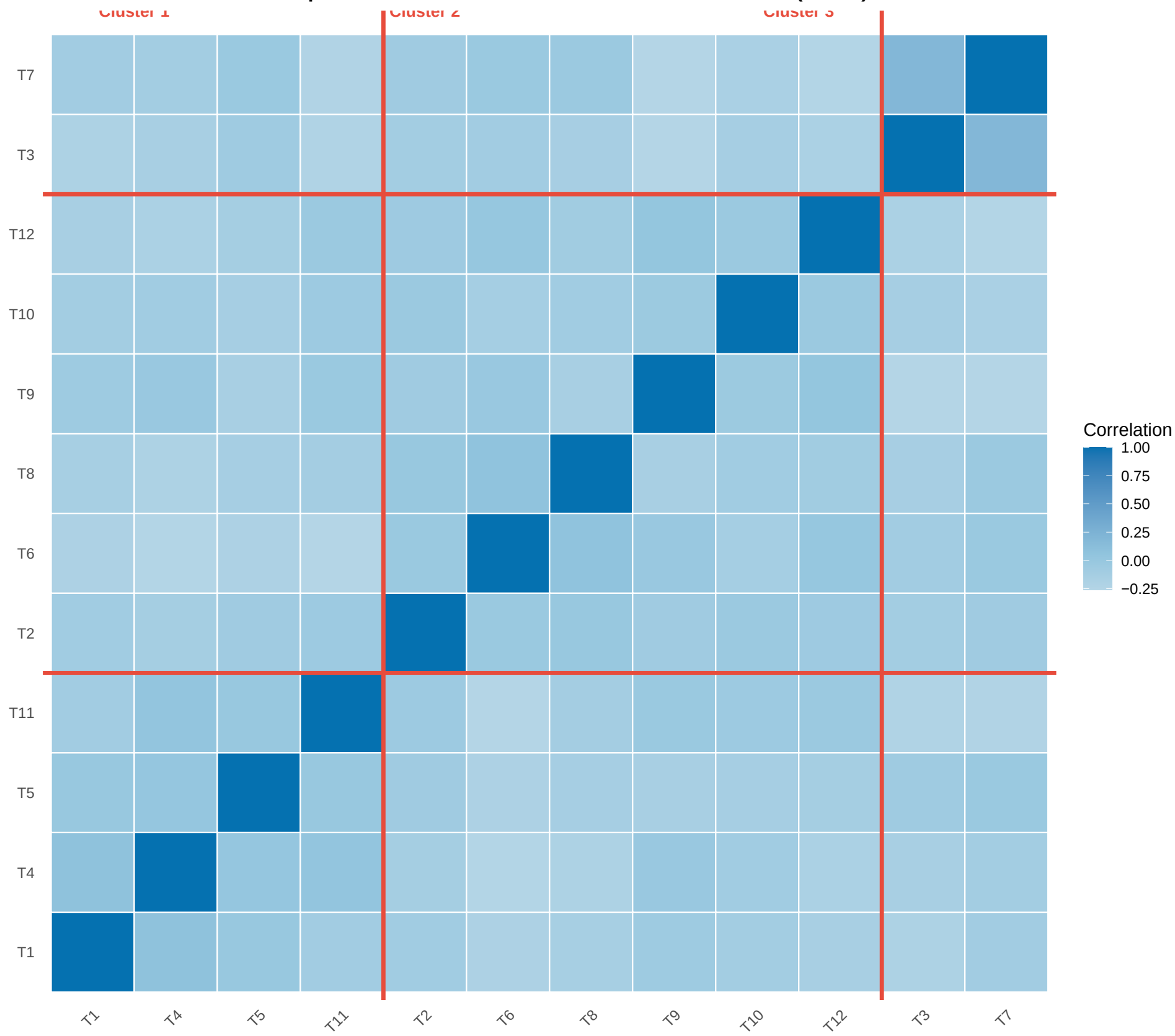
Inter-Topic Correlations with Hierarchical Cluster Structure (K = 12)
