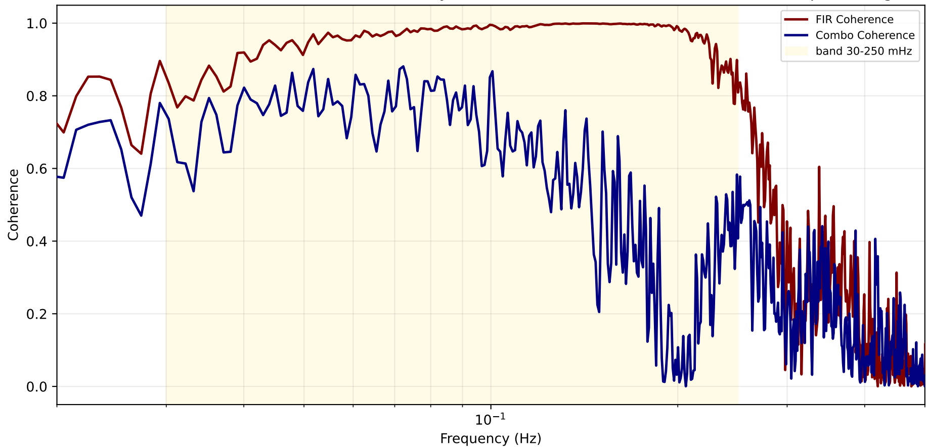
DARM — blind folder 1424689218 (Blind Noisy): Coherence of Predicted and Combo with Optical Target
