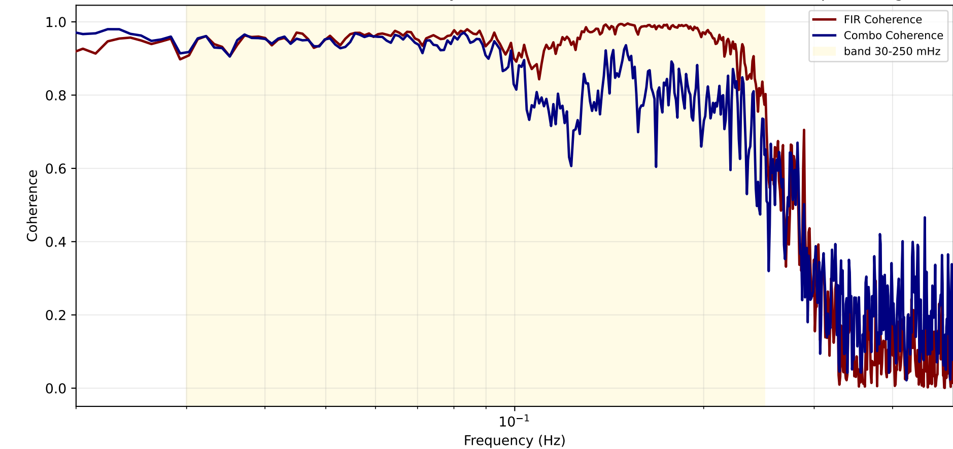
FC — blind folder 1424689218 (Blind Noisy): Coherence of Predicted and Combo with Optical Target
