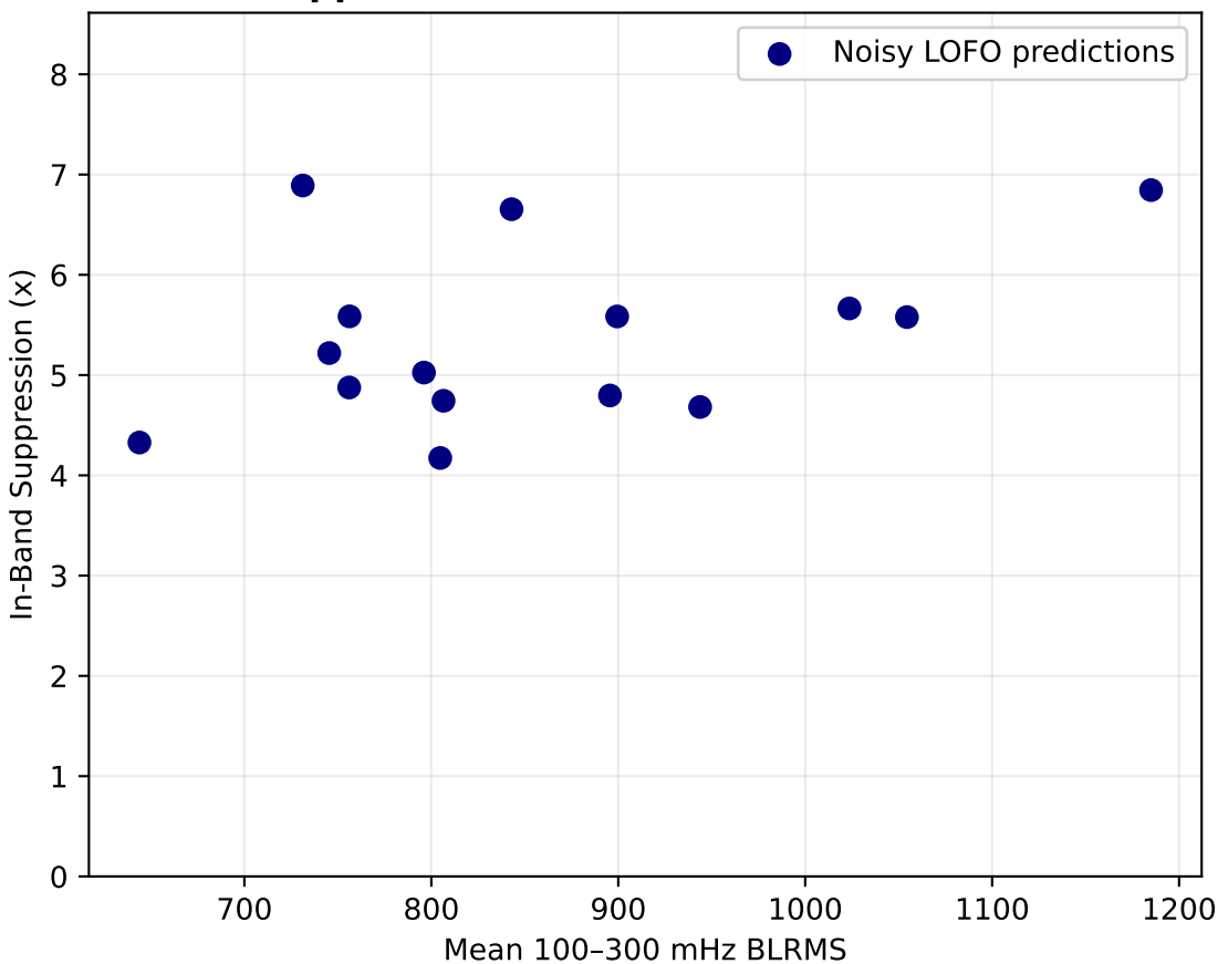
FC: Suppression vs Mean 100-300 mHz BLRMS
