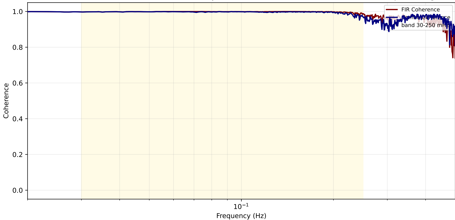
IMC — blind folder 1422266402 (Blind Noisy): Coherence of Predicted and Combo with Optical Target
