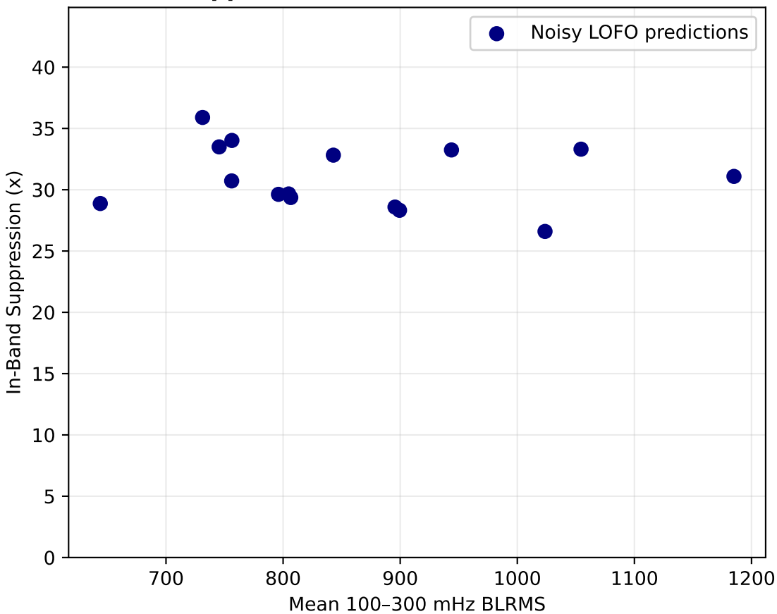
IMC: Suppression vs Mean 100-300 mHz BLRMS
