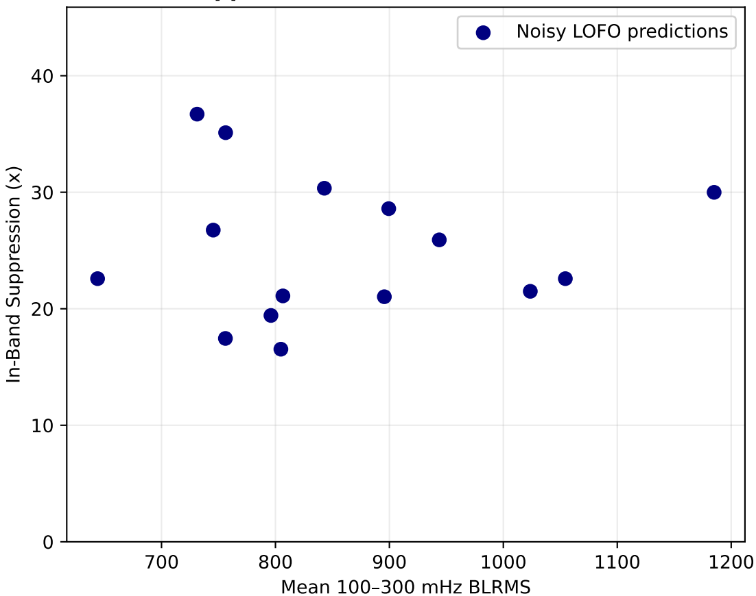
MICH: Suppression vs Mean 100-300 mHz BLRMS
