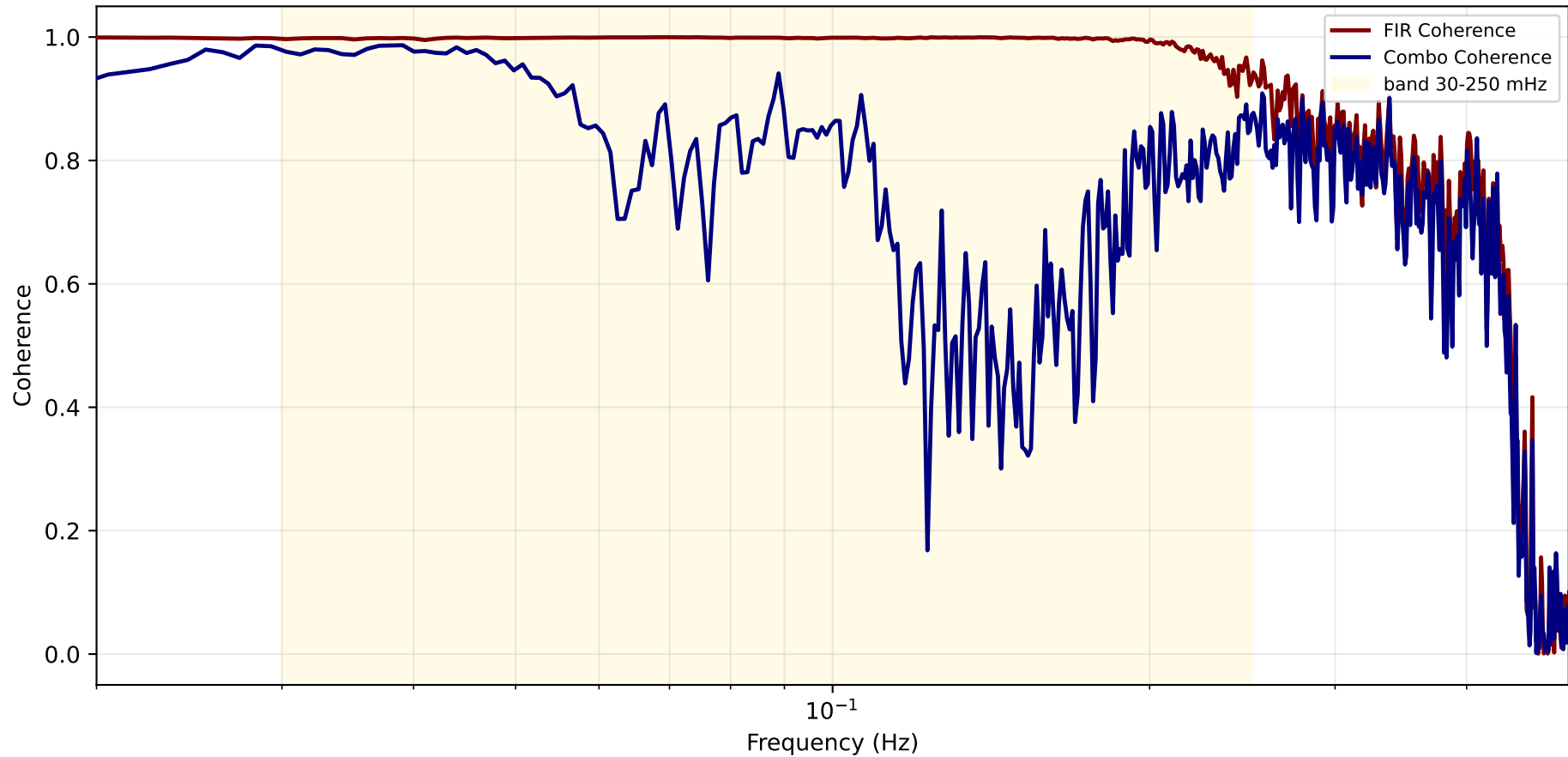
PRCL — blind folder 1422266402 (Blind Noisy): Coherence of Predicted and Combo with Optical Target
