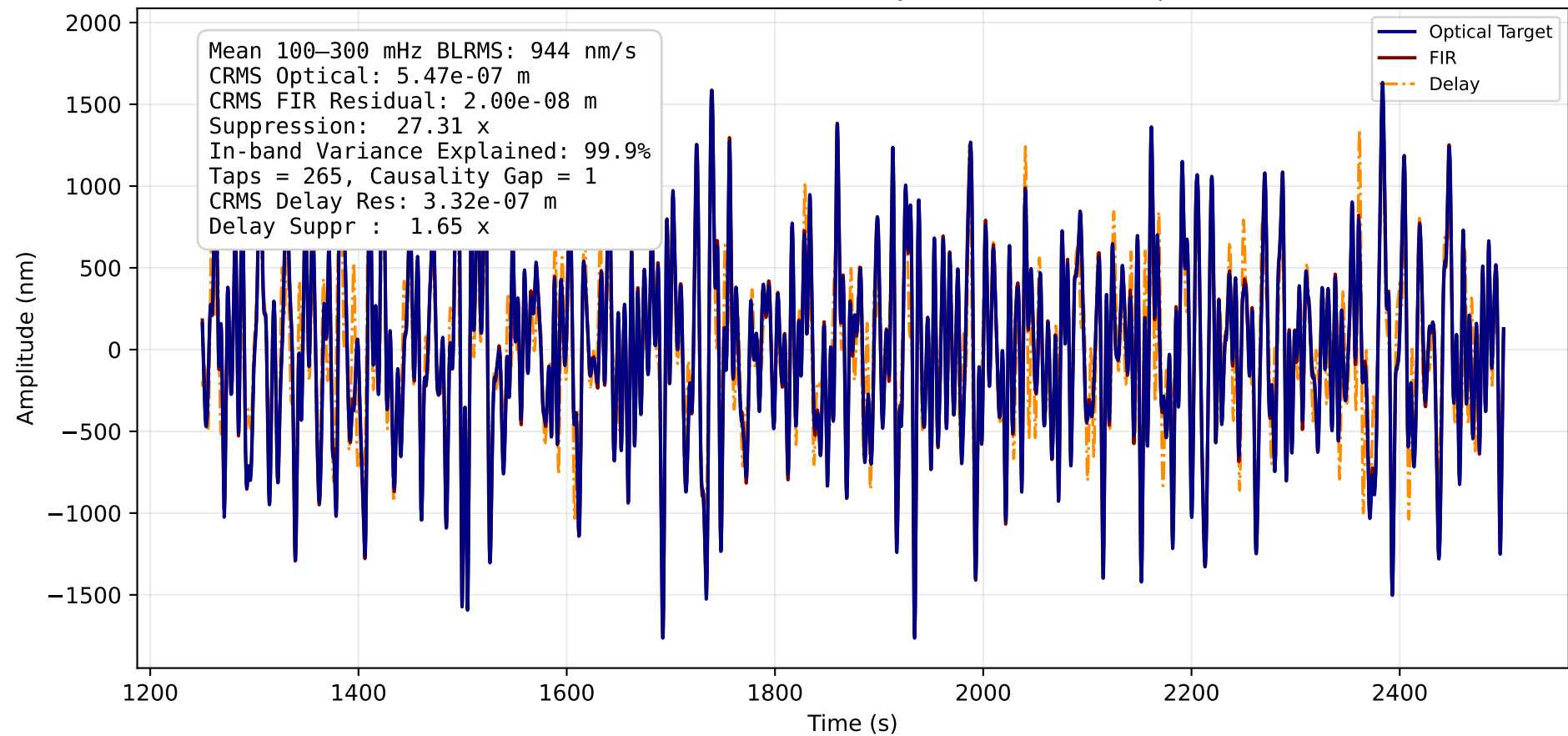
PRCL — blind folder 1422266402 (Blind Noisy): Time series of Optical vs Predicted
