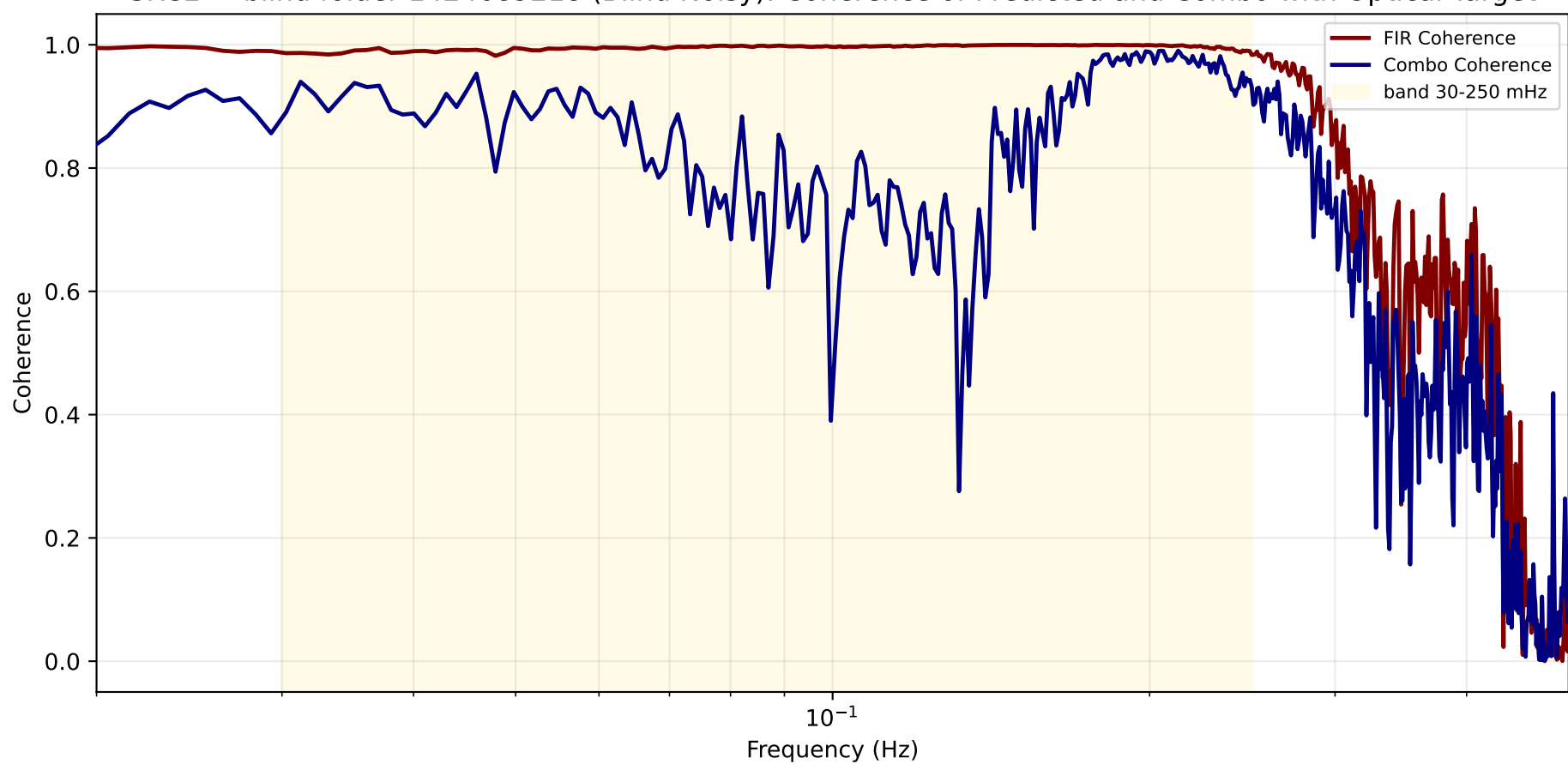
SRCL — blind folder 1424689218 (Blind Noisy): Coherence of Predicted and Combo with Optical Target
