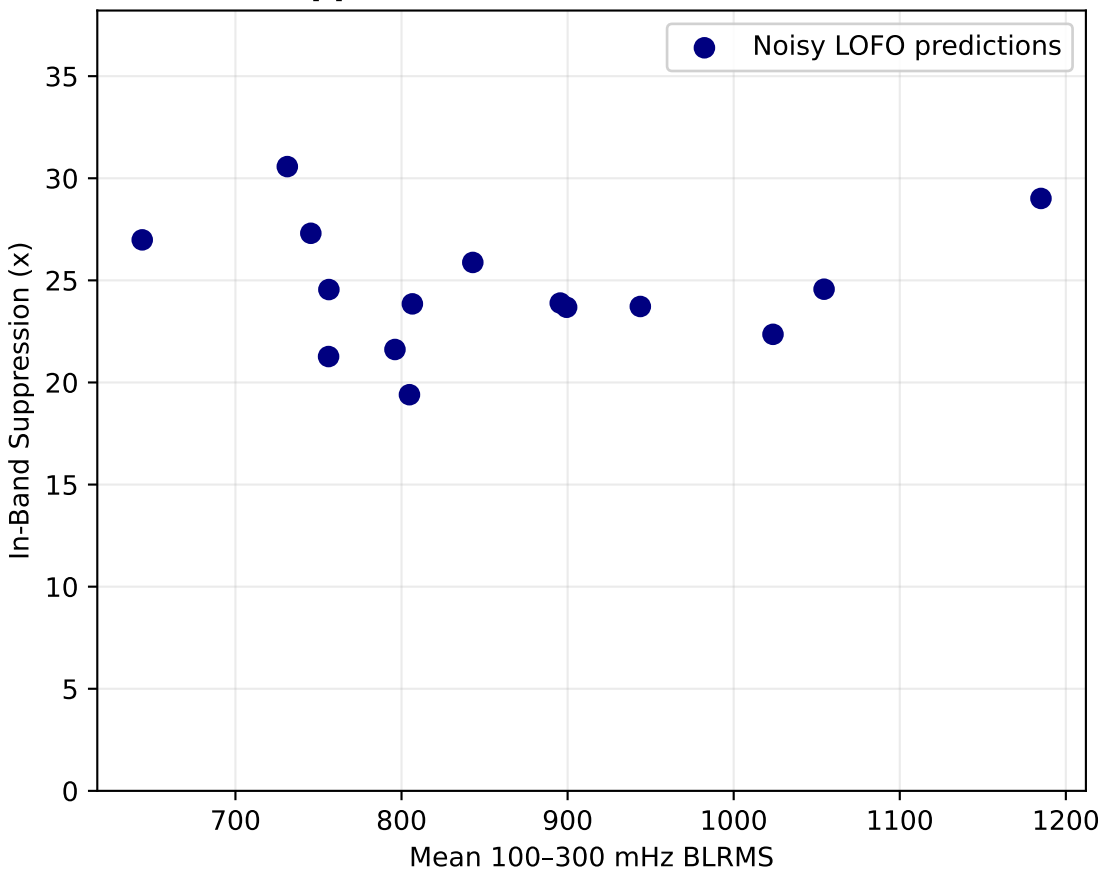
SRCL: Suppression vs Mean 100-300 mHz BLRMS
