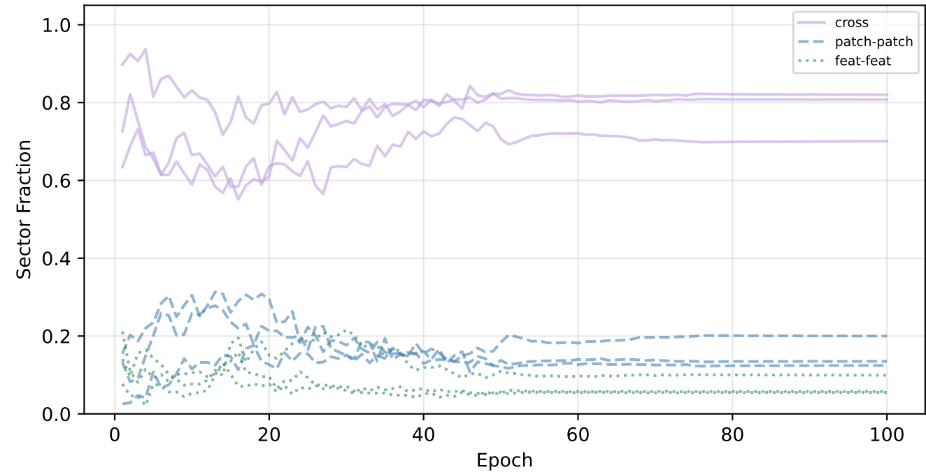
D: Compound (full sector) [butterfly, lite, train_subset_5000] — breastmnist
