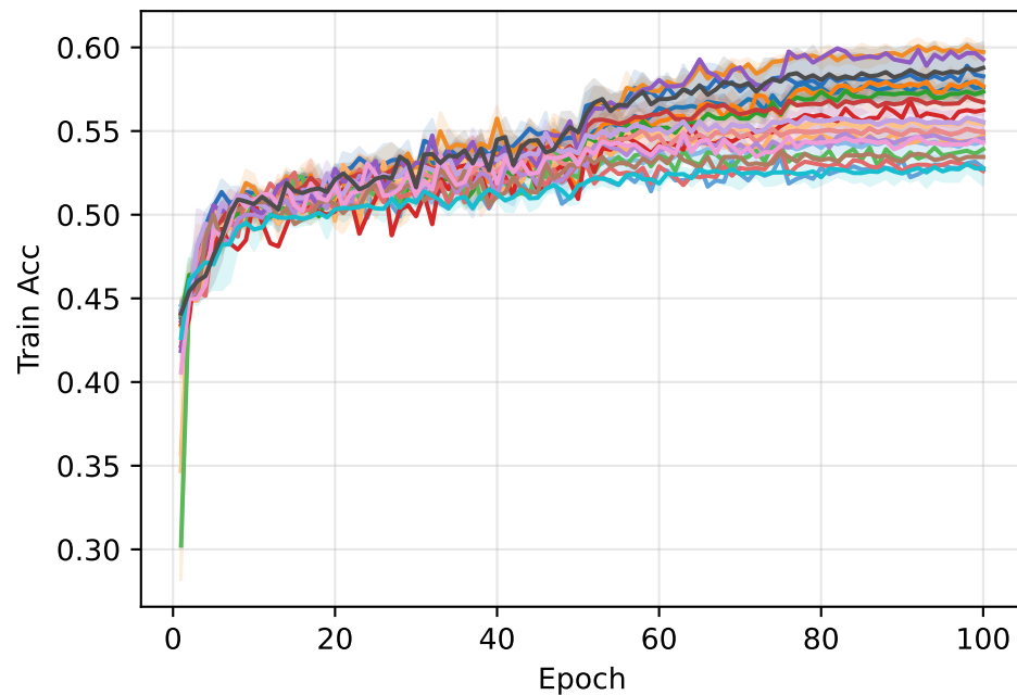
Training Curves — retinamnist
