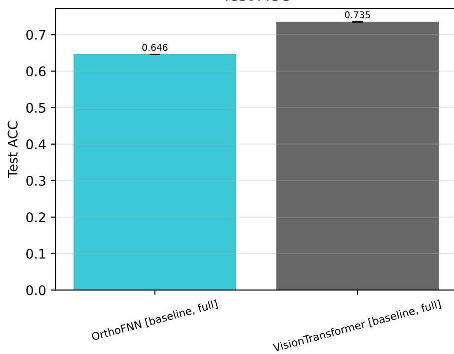
Test ACC
