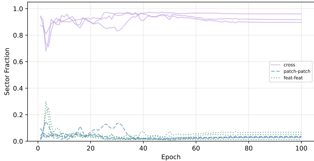
D: Compound (full sector) [butterfly, lite, train_subset_5000] — pathmnist
