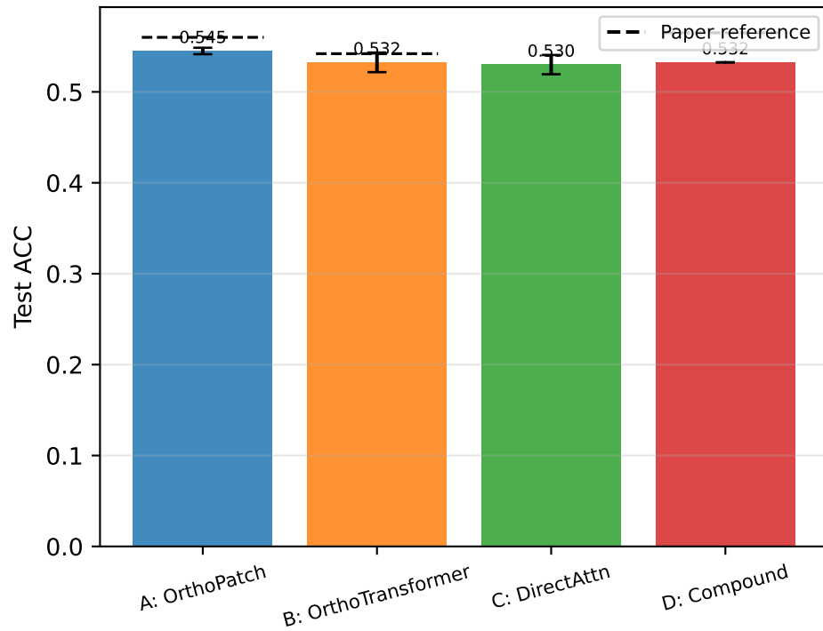
Test ACC
