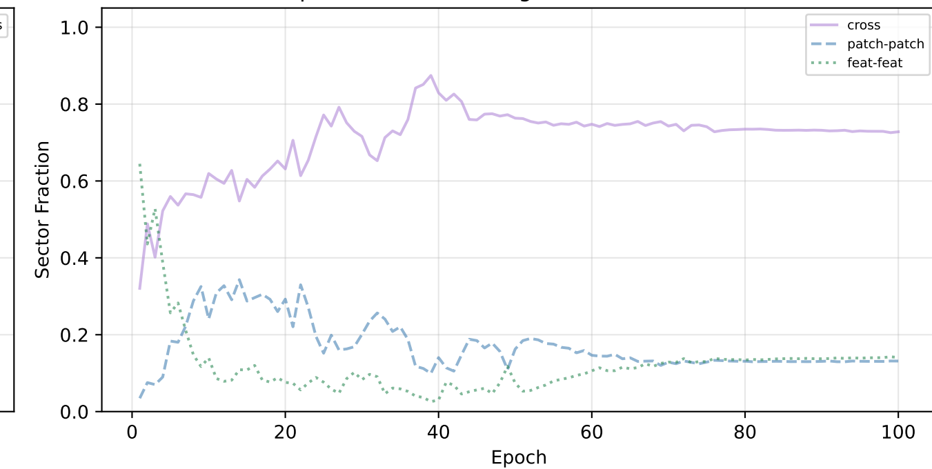
D: Compound (full sector) [generic, lite] — retinamnist
