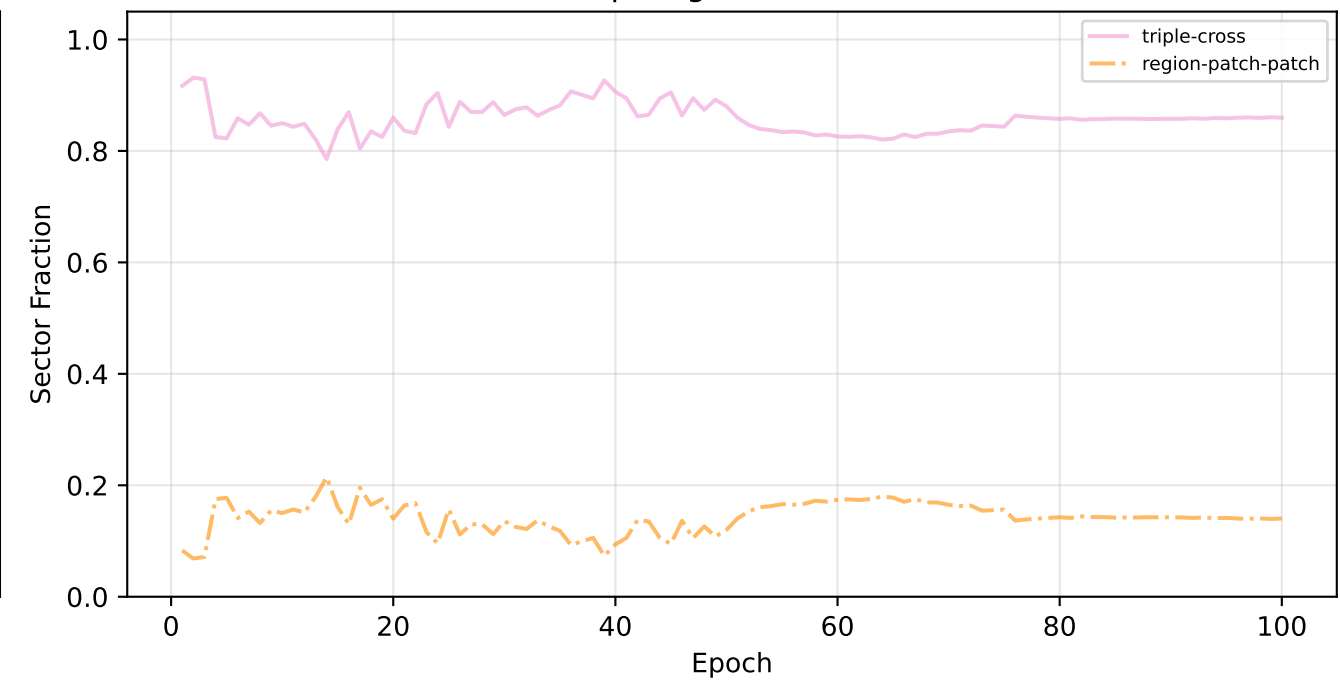
F: Hierarchical (3ph) [generic, lite] — retinamnist
