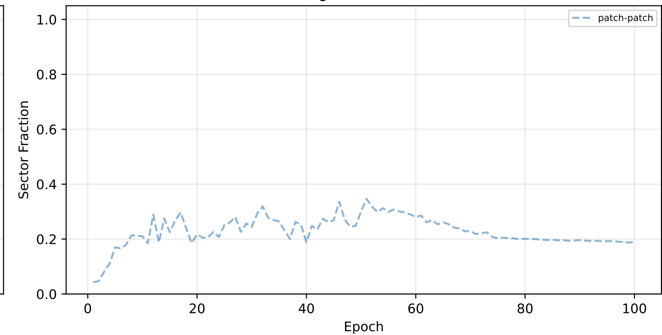
E: Multi-sector [generic, lite] — retinamnist
