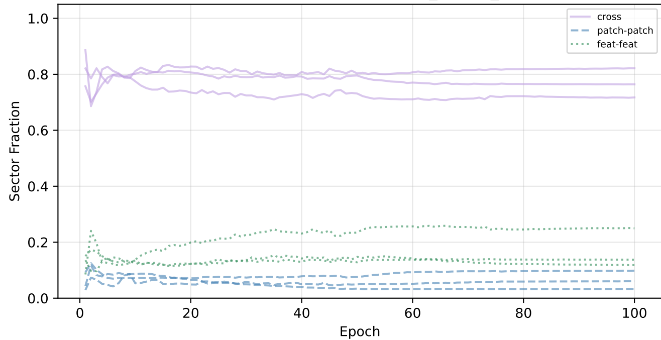
D: Compound (full sector) [butterfly, lite, train_subset_5000] — bloodmnist
