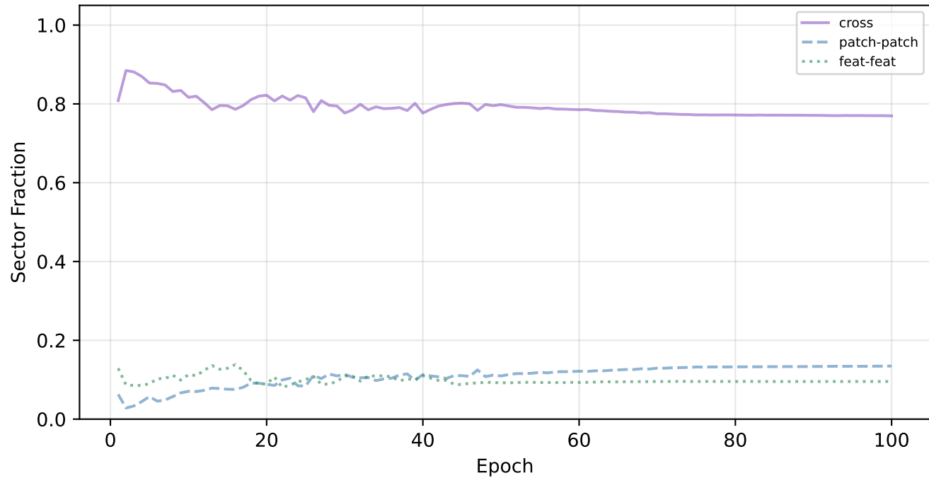
D: Compound (full sector) [butterfly, full] — retinamnist
