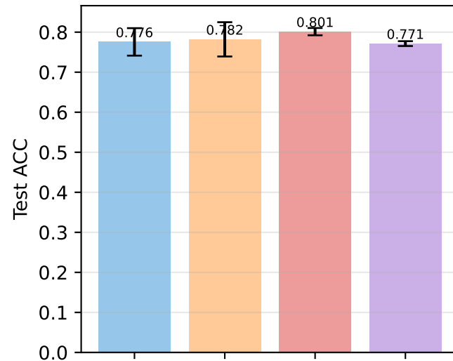
Test ACC
