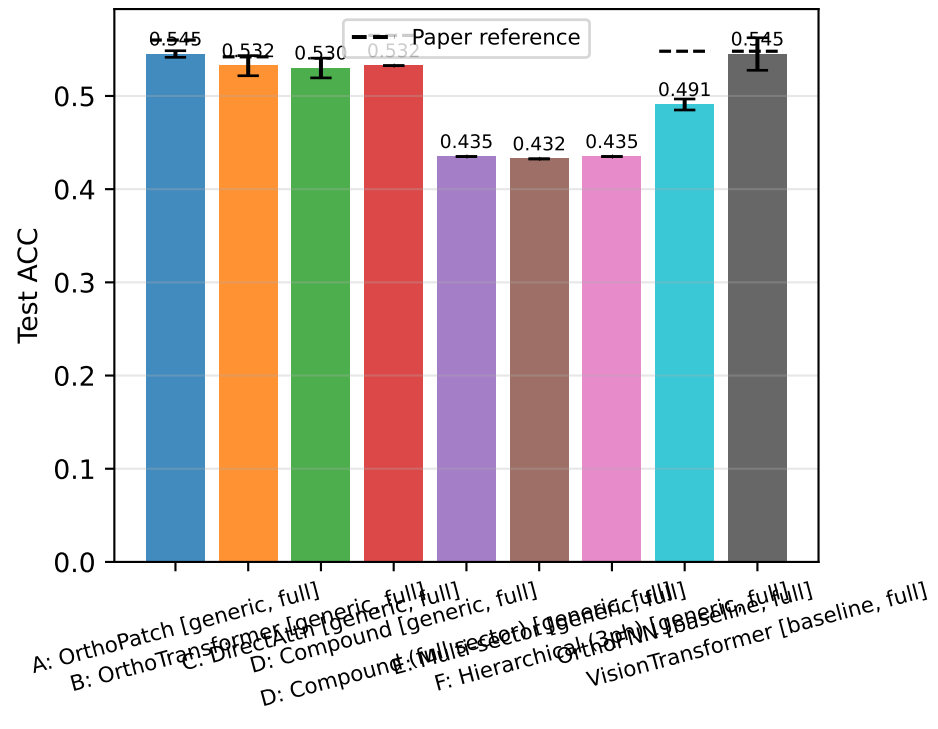
Test ACC
