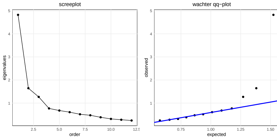
Figure 1: Screeplot and qq-plot with a fitted line.
