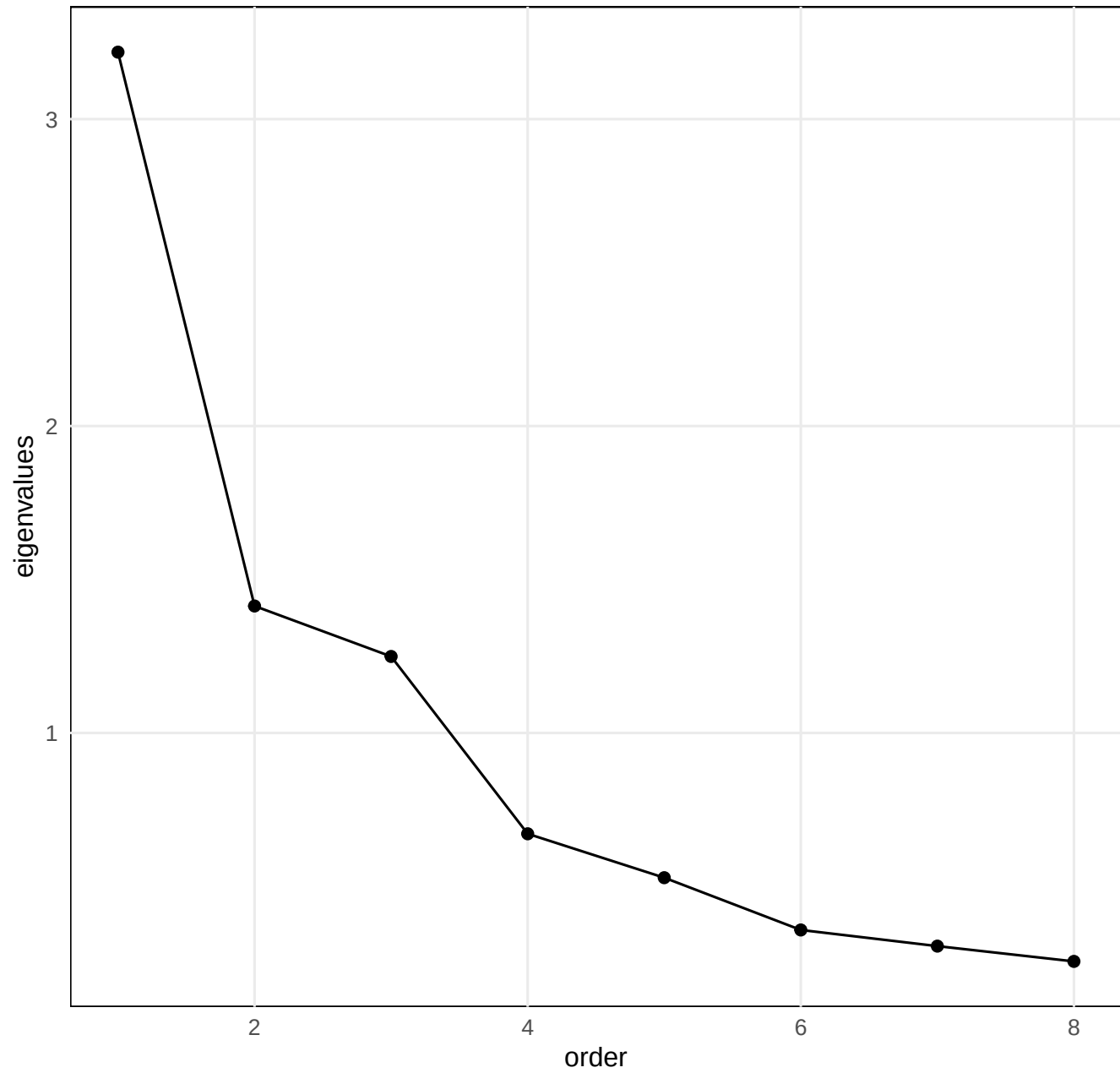
Screeplot
