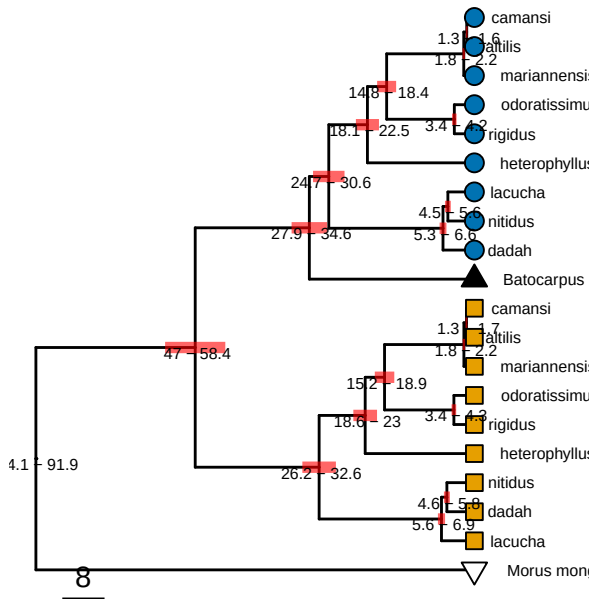
Subgenomes_4Fold.ann
