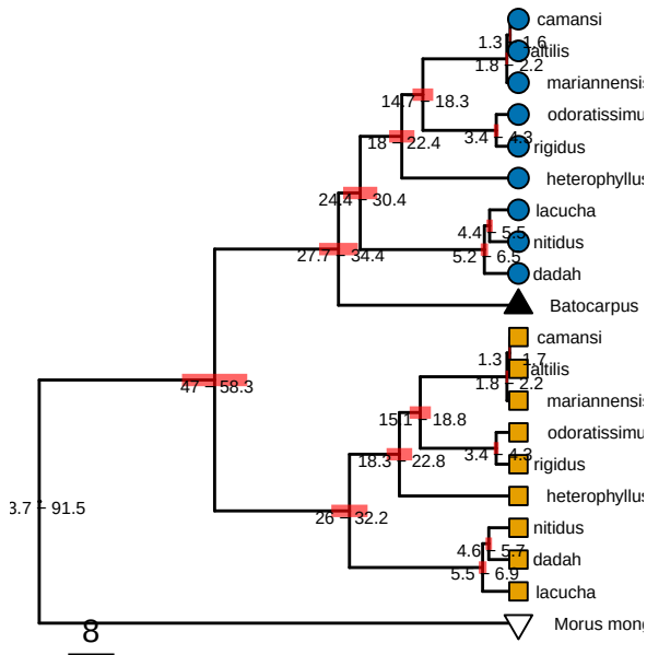
Subgenomes_4Fold_Strict.ann
