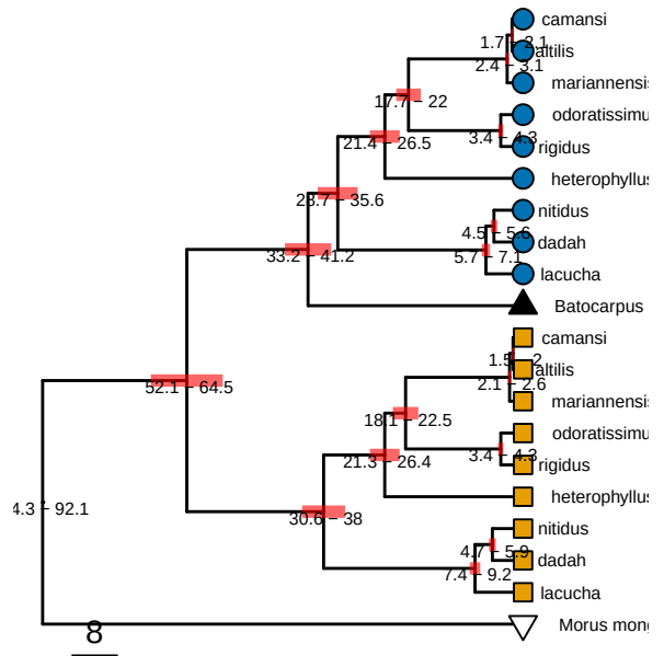
Subgenomes_FullGenes_Strict_150k.a
