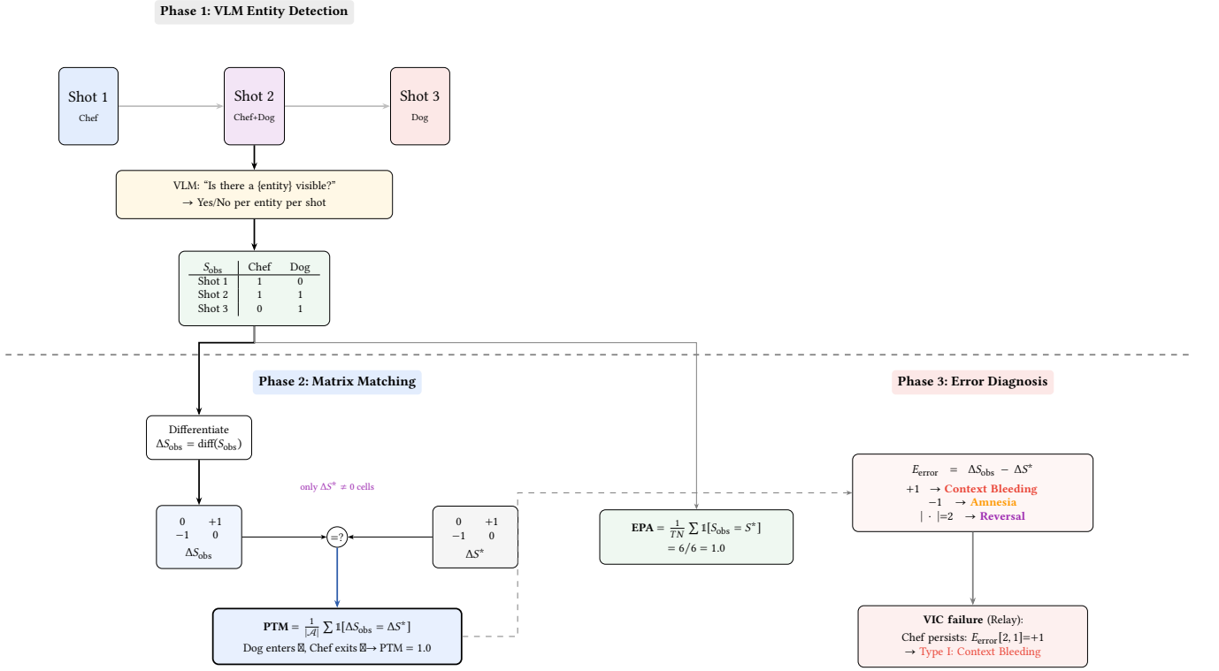
Figure 2: STEM pipeline. Phase 1: a VLM queries binary entity presence per shot, producing S_{obs} \in \{0, 1\}^{T \times N} . Phase 2: row-differencing yields \Delta S_{obs} , compared against \Delta S^* ; PTM (microscopic) evaluates prescribed cells ( \Delta S^* \neq 0 ), EPA (macroscopic) evaluates full cast compliance. Phase 3: the error matrix E = \Delta S_{obs} - \Delta S^* classifies failures into Context Bleeding, Amnesia, and Reversal.
