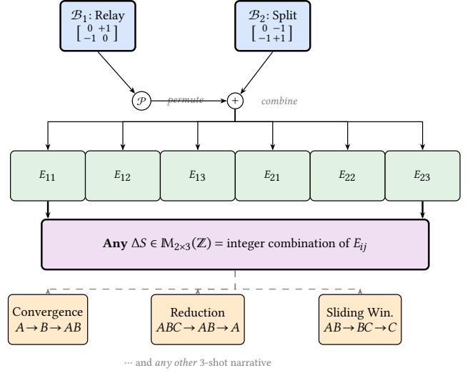
Figure 1: Completeness of the narrative space (SPAN). Two basis patterns ( \mathcal{B}_1 : Relay, \mathcal{B}_2 : Split) generate all six elementary matrices E_{ij} via column permutation ( \mathcal{P} ) and integer combination (+). Any \Delta S is a sum of E_{ij} , so the SPAN basis provably spans the entire space of 3-shot narrative topologies.
