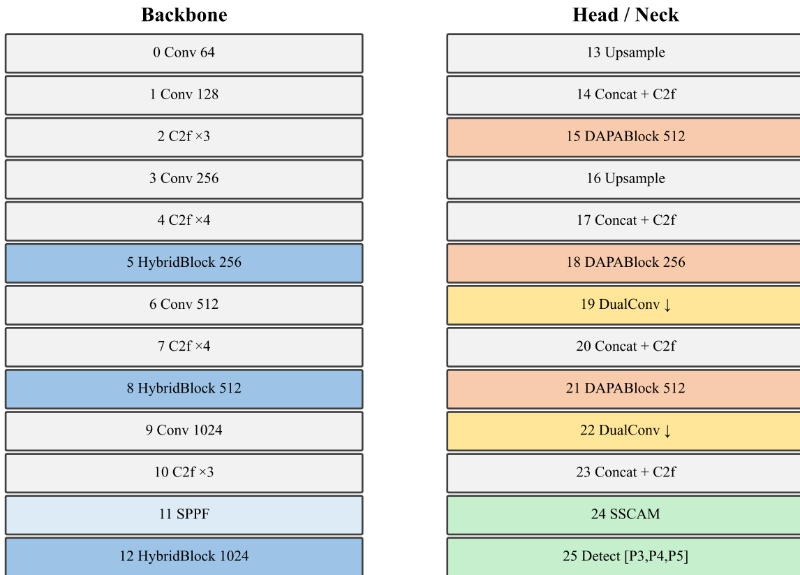
Figure 3.2 Hybrid YOLO layer / scale map
