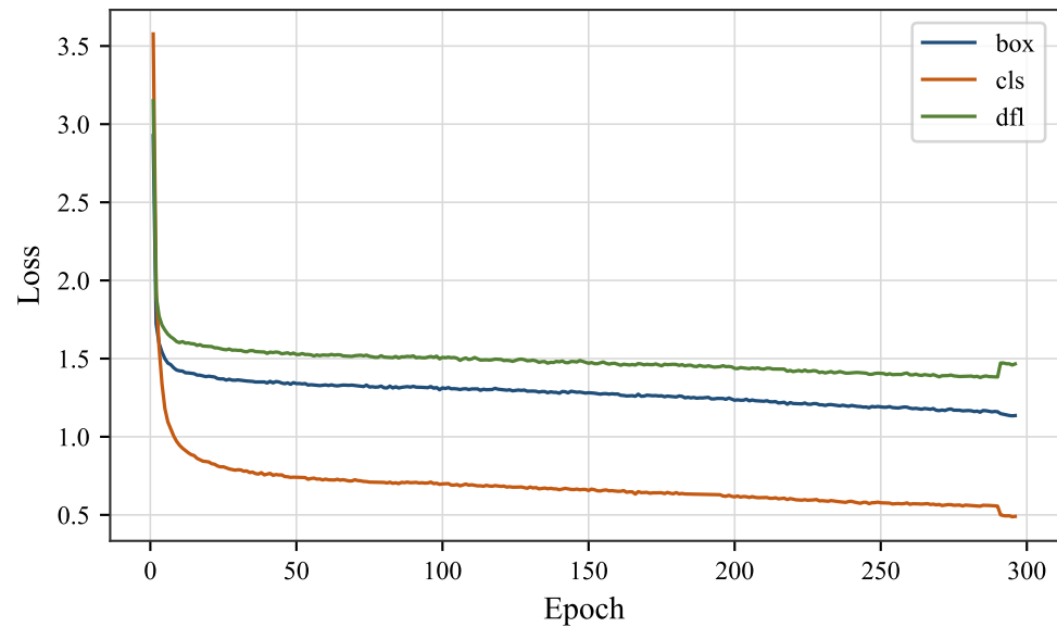
(a) Long-stage train losses
