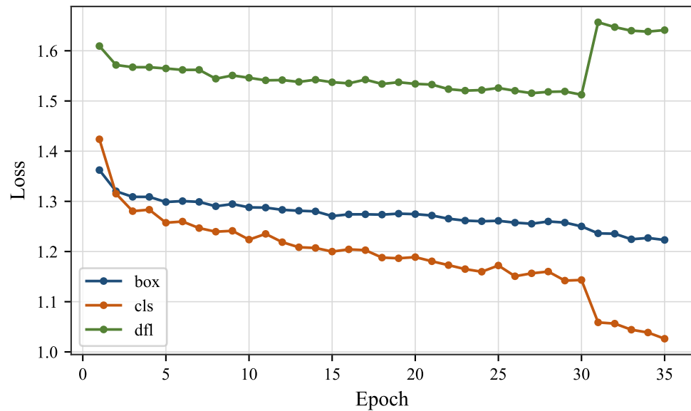
(b) Rare-FT train losses
