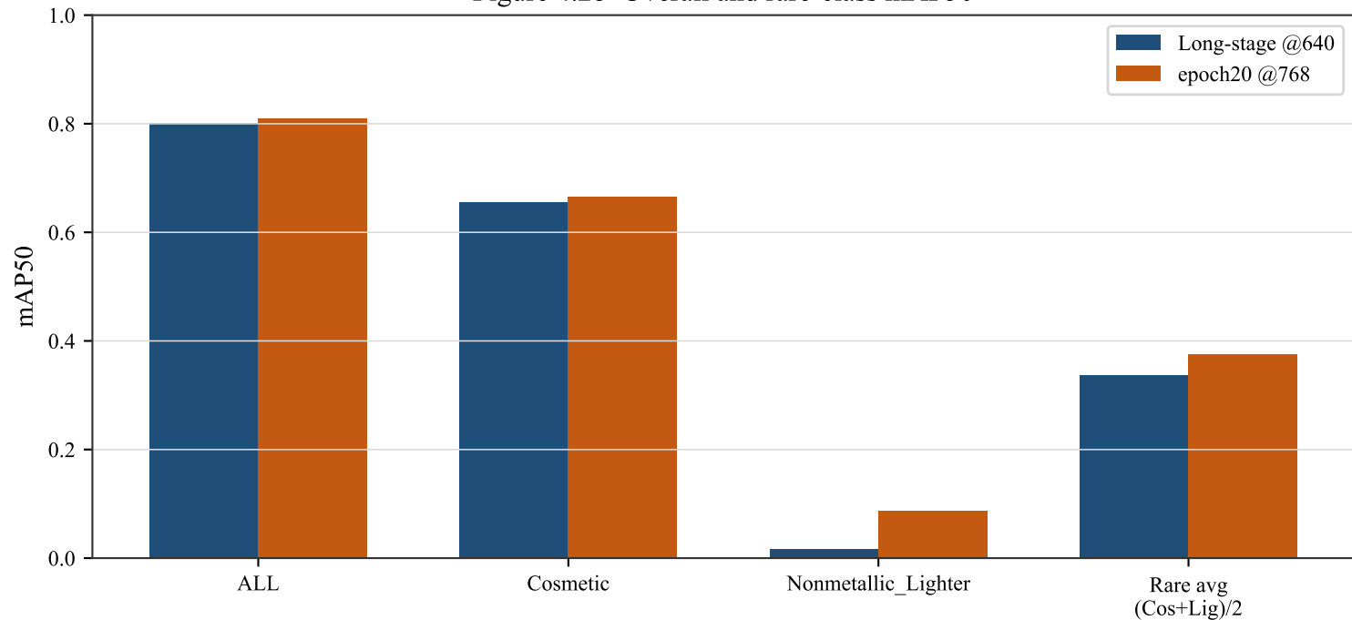
Figure 4.2b Overall and rare-class mAP50
