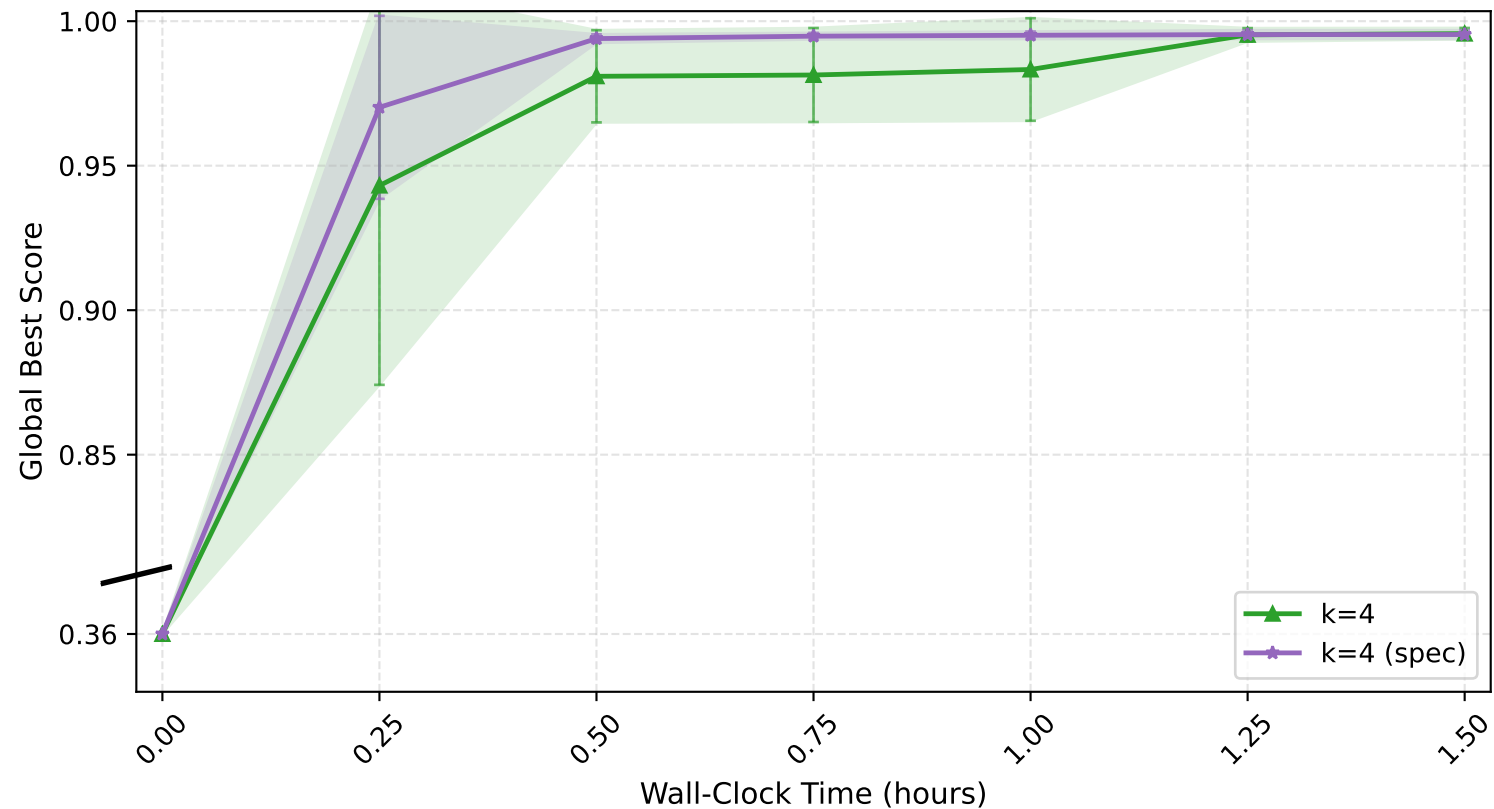
Circle Packing — Best Score vs Wall-Clock Time k=4 vs k=4 (spec) | mean \pm std over 3 runs
