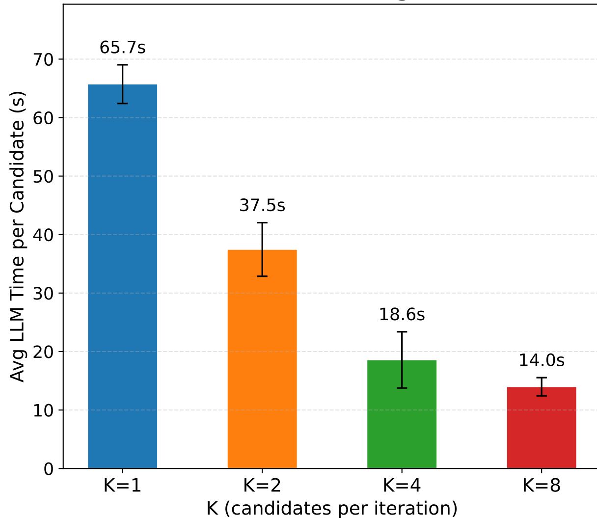
Circle Packing
