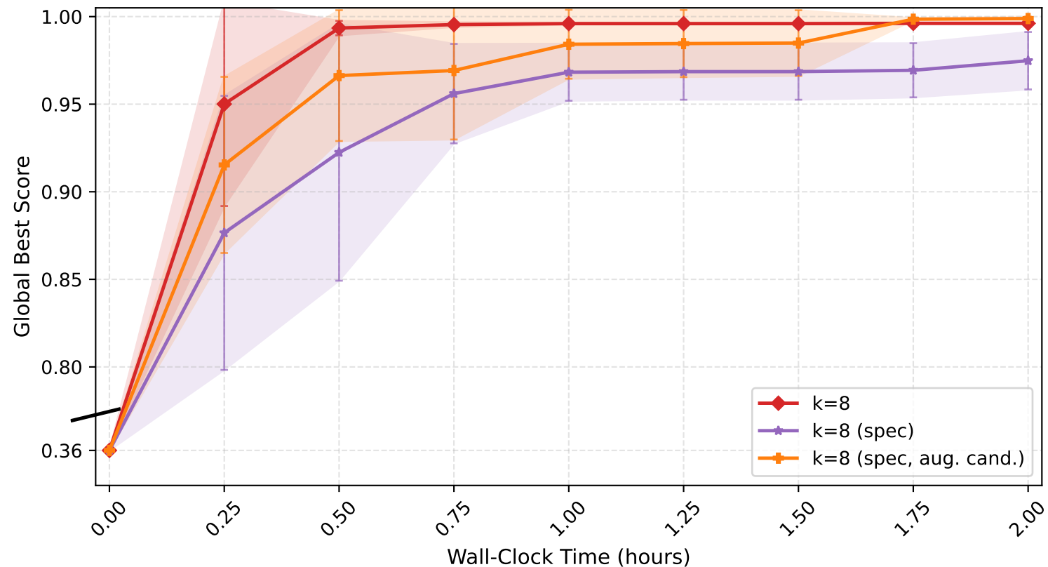
Circle Packing — Best Score vs Wall-Clock Time k=8 vs k=8 (spec) | mean \pm std over 3 runs
