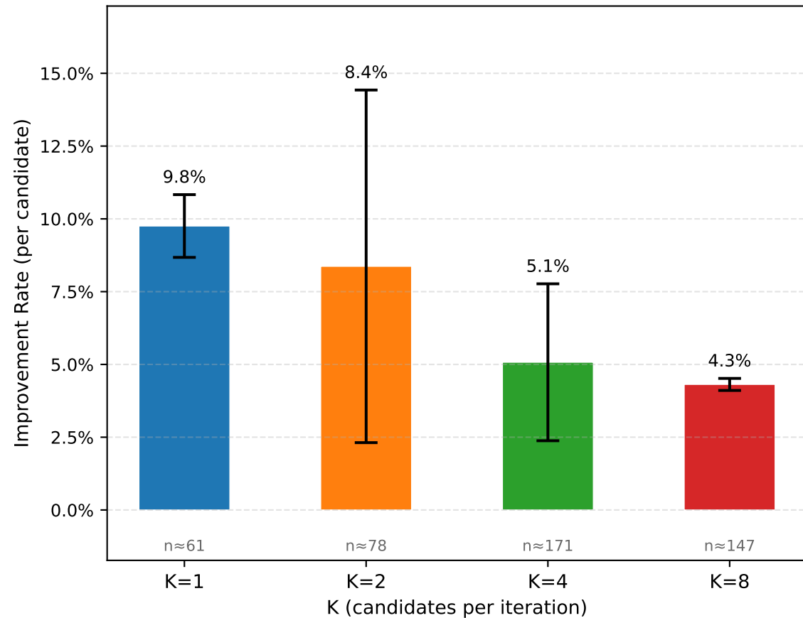
Circle Packing
