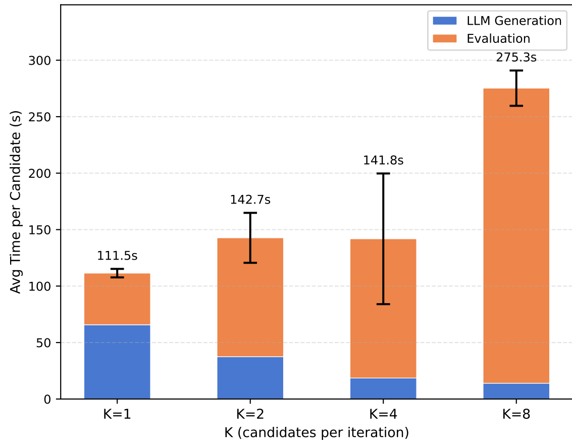
Circle Packing
