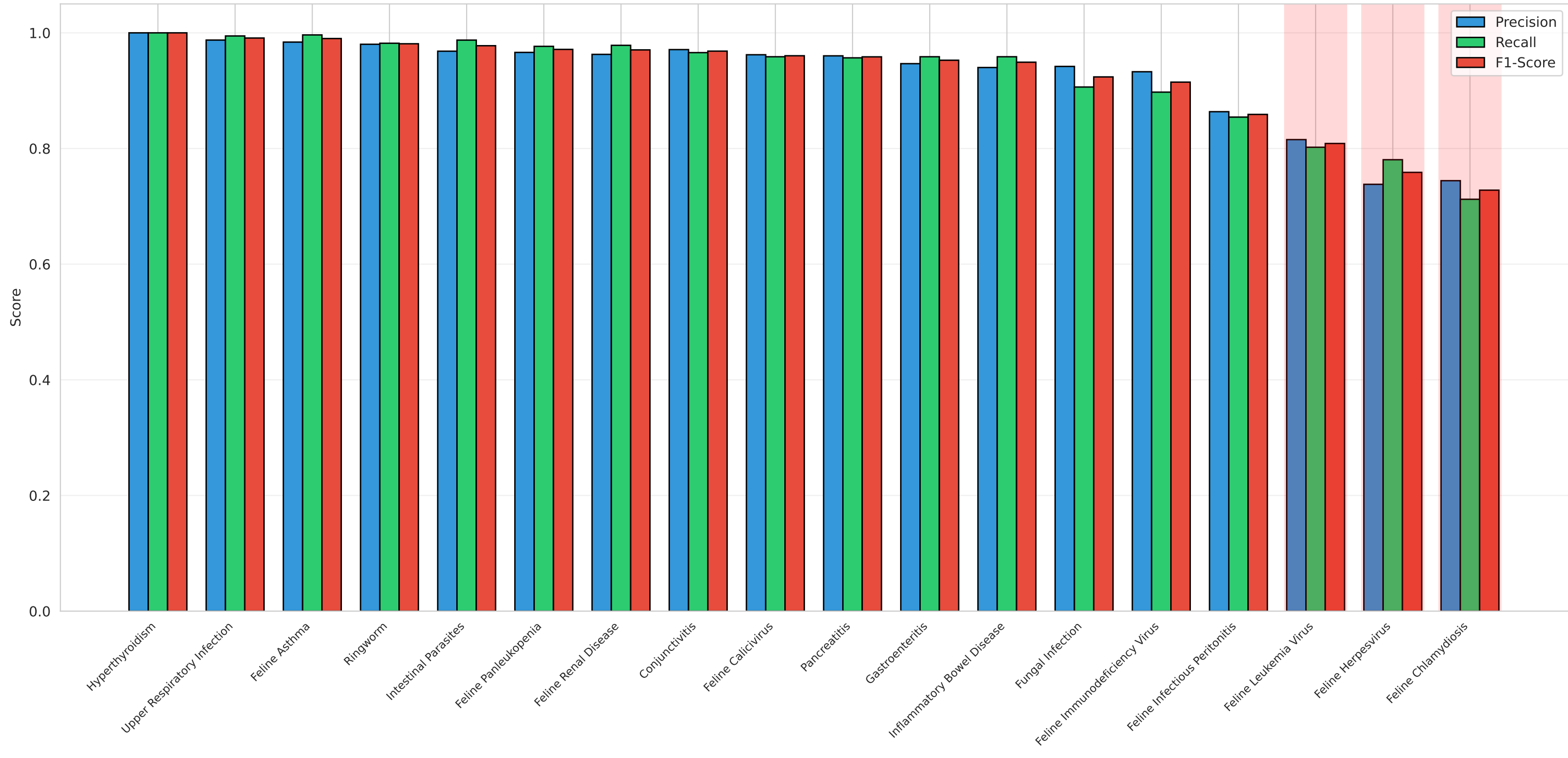
Per-Class Performance (sorted by F1) — Stacking_All_Top5
