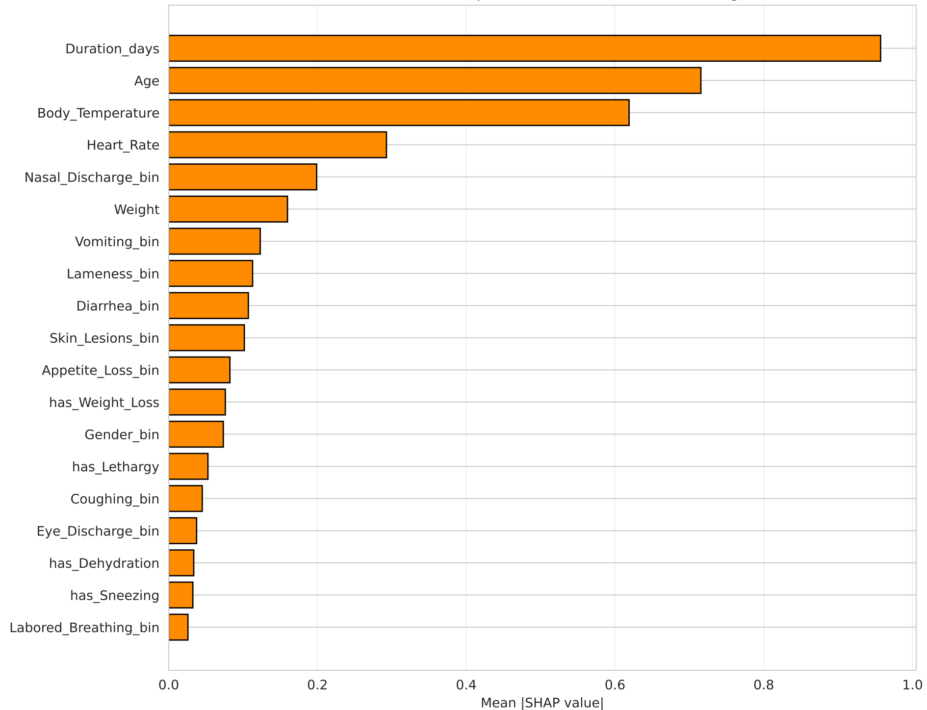
SHAP Feature Importance — HistGradientBoosting
