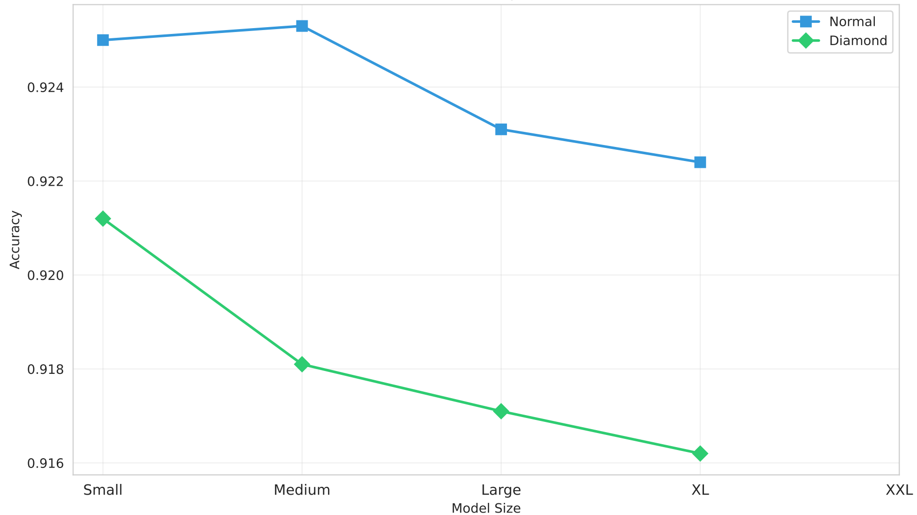
Size Effect on Accuracy (MLP variants)
