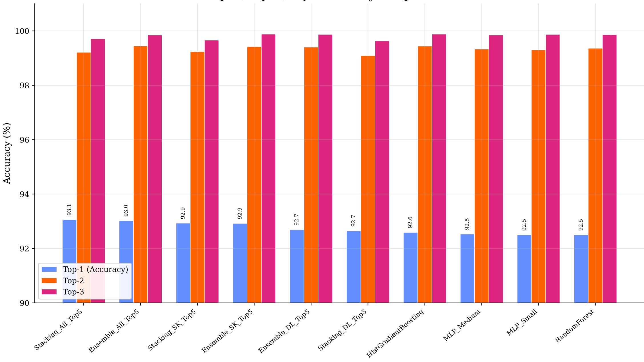
Top-1 / Top-2 / Top-3 Accuracy — Top 10 Models
