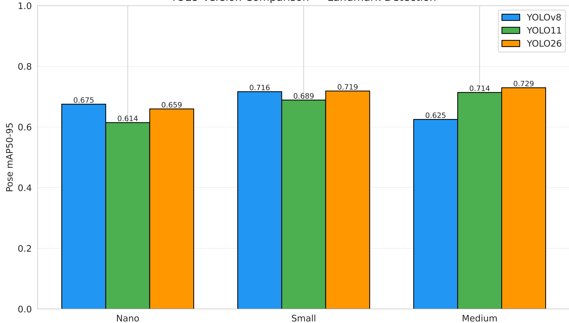
YOLO Version Comparison — Landmark Detection
